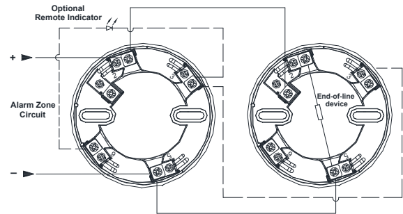
Fig. 1: 2-wire base wiring connections
