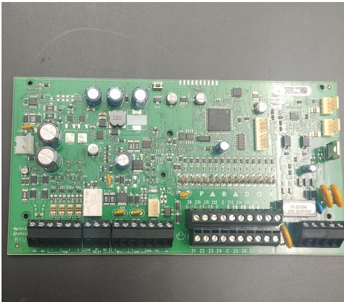
Photograph 5.1.4, 5.1.5 -PCB view
