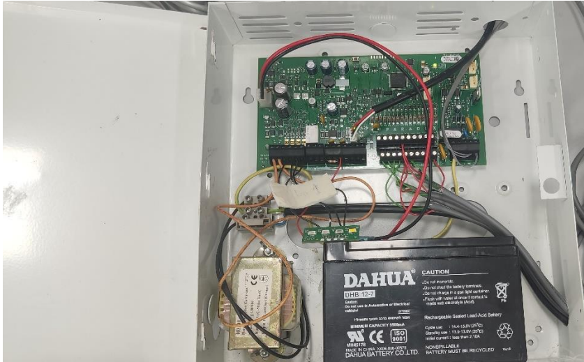
Photograph 5.1.3 - Internal view
