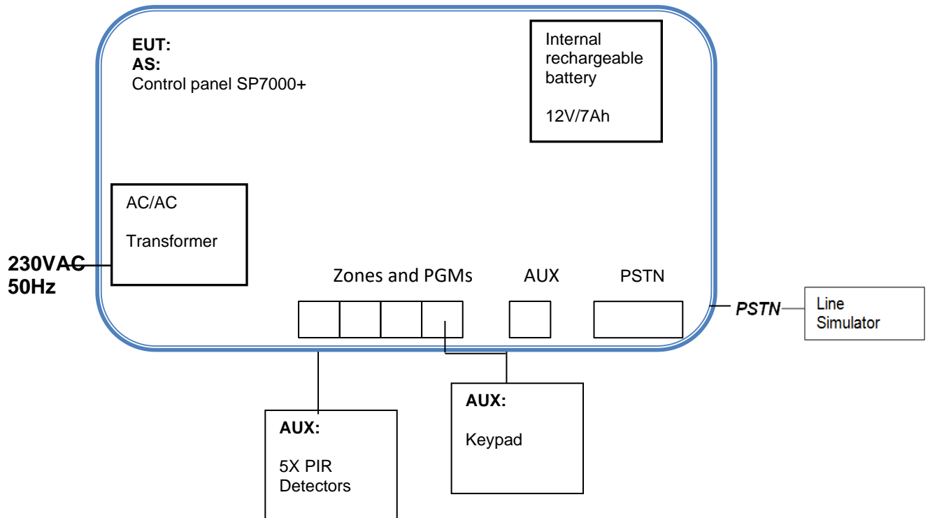
Figure 5.2.1 Setup configuration
