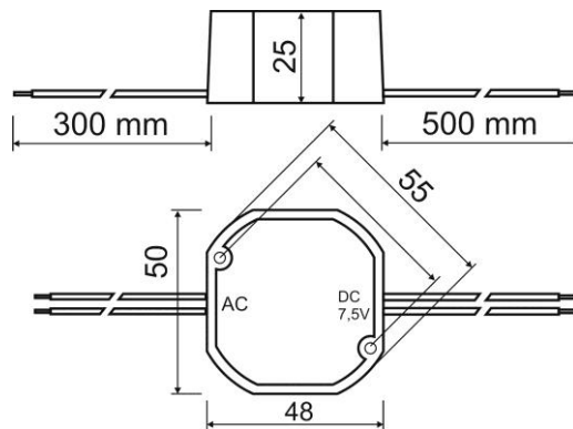
Fig.1. Mechanical view and dimensions of the PSU.
