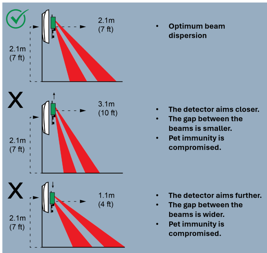
Device Board Height Adjustments
